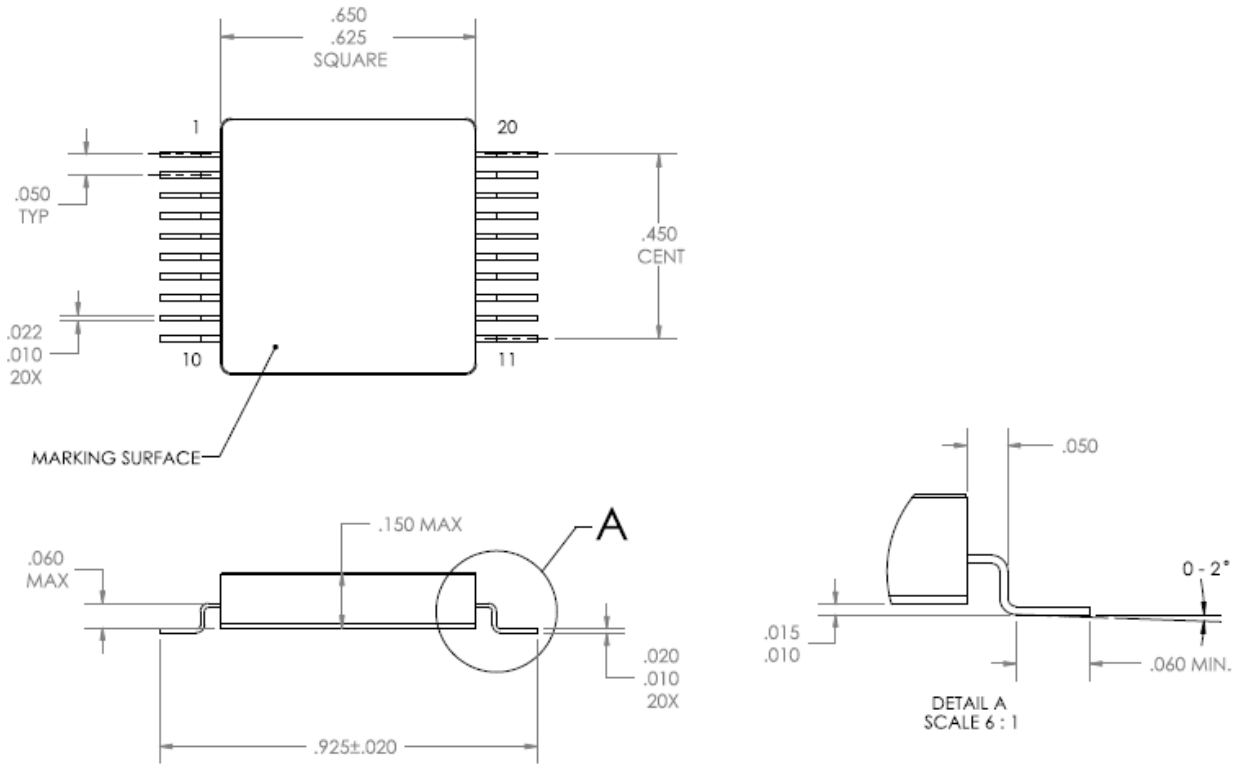
FIGURE 2 Models 1420 Package Outline
