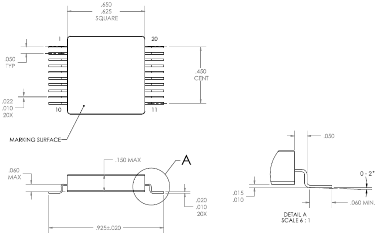
FIGURE 2 Models 1520 Package Outline
