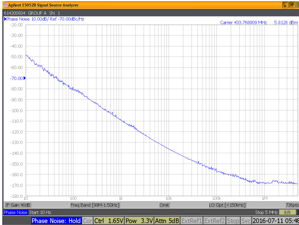
Figure 1A – Typical Phase Noise @ 433.768MHz
