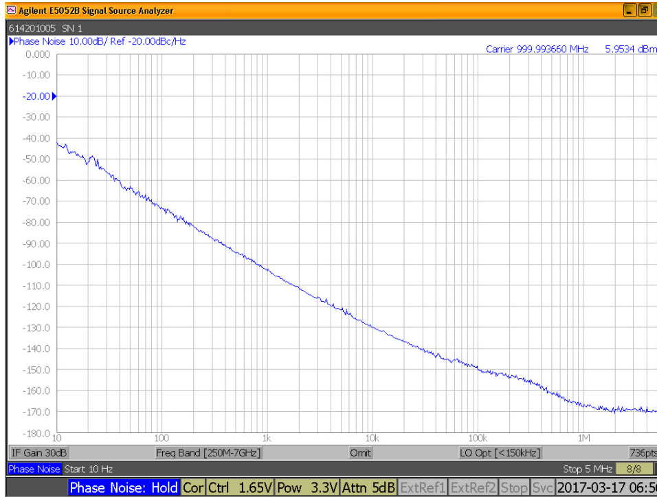
Figure 1C – Typical Phase Noise @ 1.000GHz
