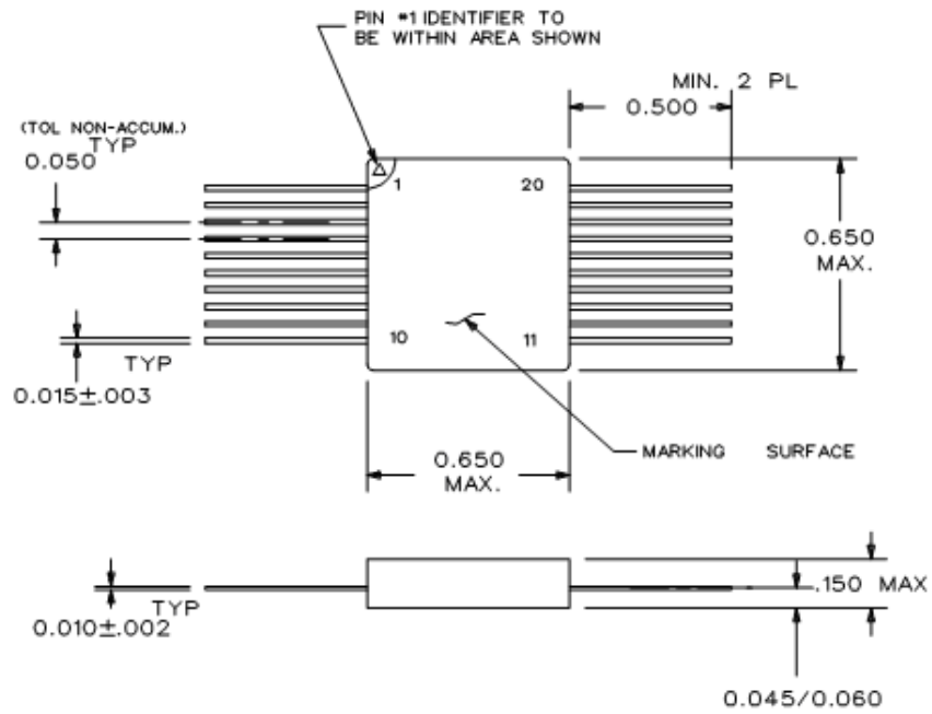
FIGURE 2 Model 6504 Package Outline
