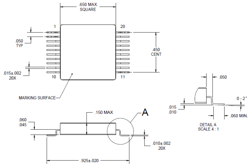
FIGURE 3 Model 6520 Package Outline
