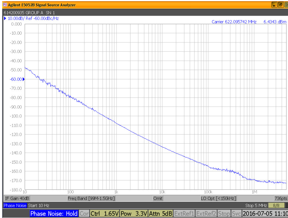
Figure 1B – Typical Phase Noise @ 622.080MHz
